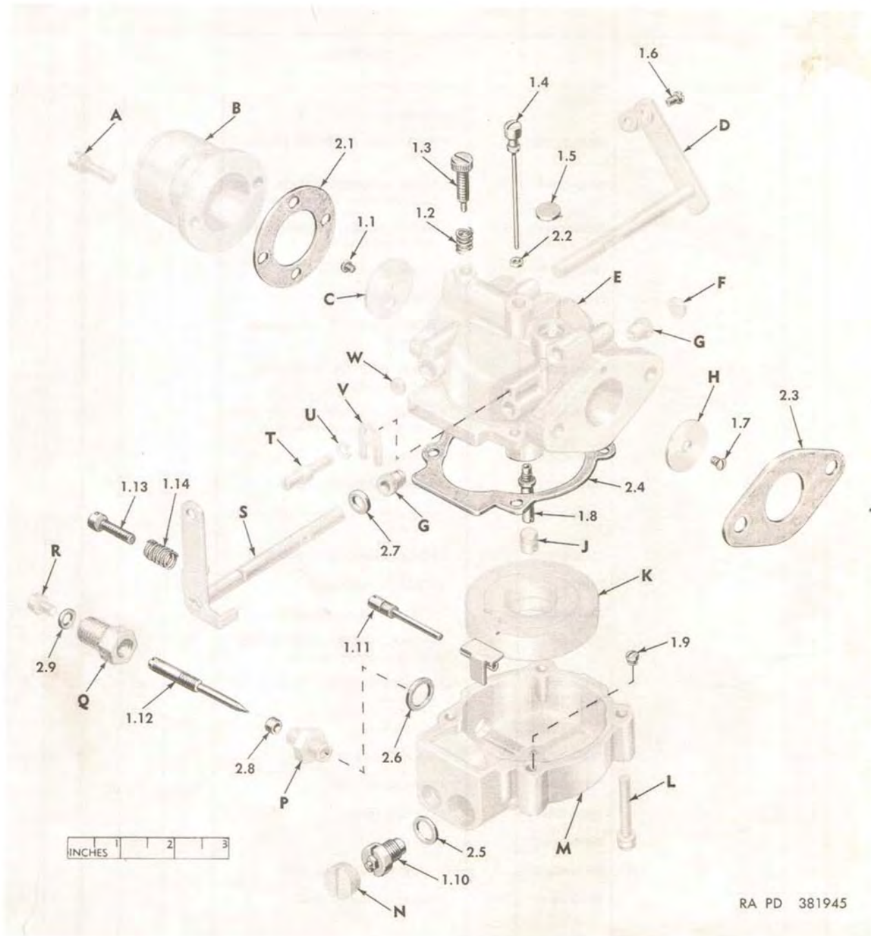
Figure 2. Carburetor, Float: Assembly - exploded view.
